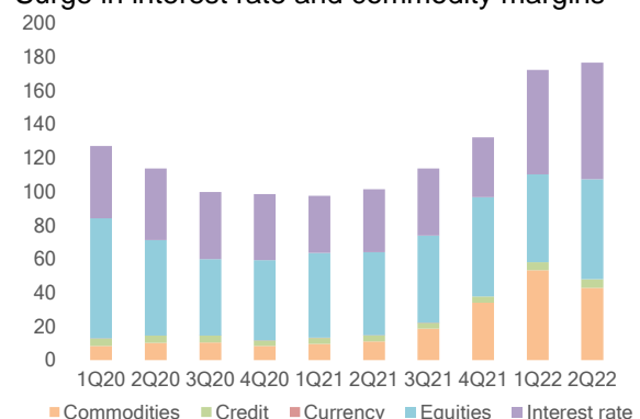
Chart 35 Initial margins collected by EU CCPs by asset class Surge in interest rate and commodity margins
